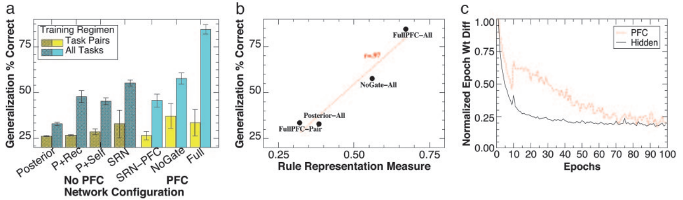
Fig. 3. Generalization and learning results. (a) Crosstask generalization results (% correct on task-novel stimuli) for the full PFC network and a variety of control networks, with either only two tasks (Task Pairs) or all four tasks (All Tasks) used during training ( n = 10 for each network, error bars are standard errors). Overall, the full PFC model generalizes substantially better than the other models, and this interacts with the level of training such that performance on the All Tasks condition is substantially better than the Task Pairs condition (with no differences in numbers of training trials or training stimuli). With one feature left out of training for each of four dimensions, training represented only 31.6% (324) of the total possible stimulus inputs (1,024); the \approx 85\% generalization performance on the remaining test items therefore represents good productive abilities. The other networks are: Posterior, a single large hidden unit layer between inputs and response, a simple model of posterior cortex without any special active maintenance abilities; P + Rec, posterior + full recurrent connectivity among hidden units, allows hidden layer to maintain information over time via attractor dynamics; P + Self, posterior + self-recurrent connections from hidden units to themselves, allows individual units to maintain activations over time; SRN, simple recurrent network, with a context layer that is a copy of the hidden layer on the prior step, a widely used form of temporal maintenance; SRN-PFC, an SRN context layer applied to the PFC layer in the full model (identical to the full PFC model except for this difference), tests for role of separated hidden layers; NoGate, the full PFC model without the AG adaptive gating unit. (b) The correlation of generalization performance with the extent to which the units distinctly and orthogonally encode stimulus dimensions for the networks shown in Fig. 2. This was computed by comparing each unit's pattern of weights to the set of five orthogonal, complete dimensional target patterns (i.e., the A dimension target pattern has a 1 for each A feature, and 0s for the features in all other dimensions, etc.). A numeric value between 0 and 1, where 1 represents a completely orthogonal and complete dimensional representation was computed for unit i as: d_i = \max_k |w_i t_k| / \sum_k |w_i t_k| ; where t_k is the dimensional target pattern k , and w_i is the weight vector for unit i , and |w_i t_k| represents the normalized dot product of the two vectors (i.e., the cosine). This value was then averaged across all units in the layer and then correlated with that network's generalization performance. (c) Relative stability of PFC and hidden layer (posterior cortex) in the model, as indexed by Euclidean distance between weight states at the end of subsequent epochs (epoch = 2,000 trials). The PFC takes longer to stabilize (i.e., exhibits greater levels of weight change across epochs) than the posterior cortex. For PFC, within-PFC recurrent weights were used. For Hidden, weights from stimulus input to Hidden were used. Both sets of weights are an equivalent distance from error signals at the output layer. The learning rate is reduced at 10 epochs, producing a blip at that point.
